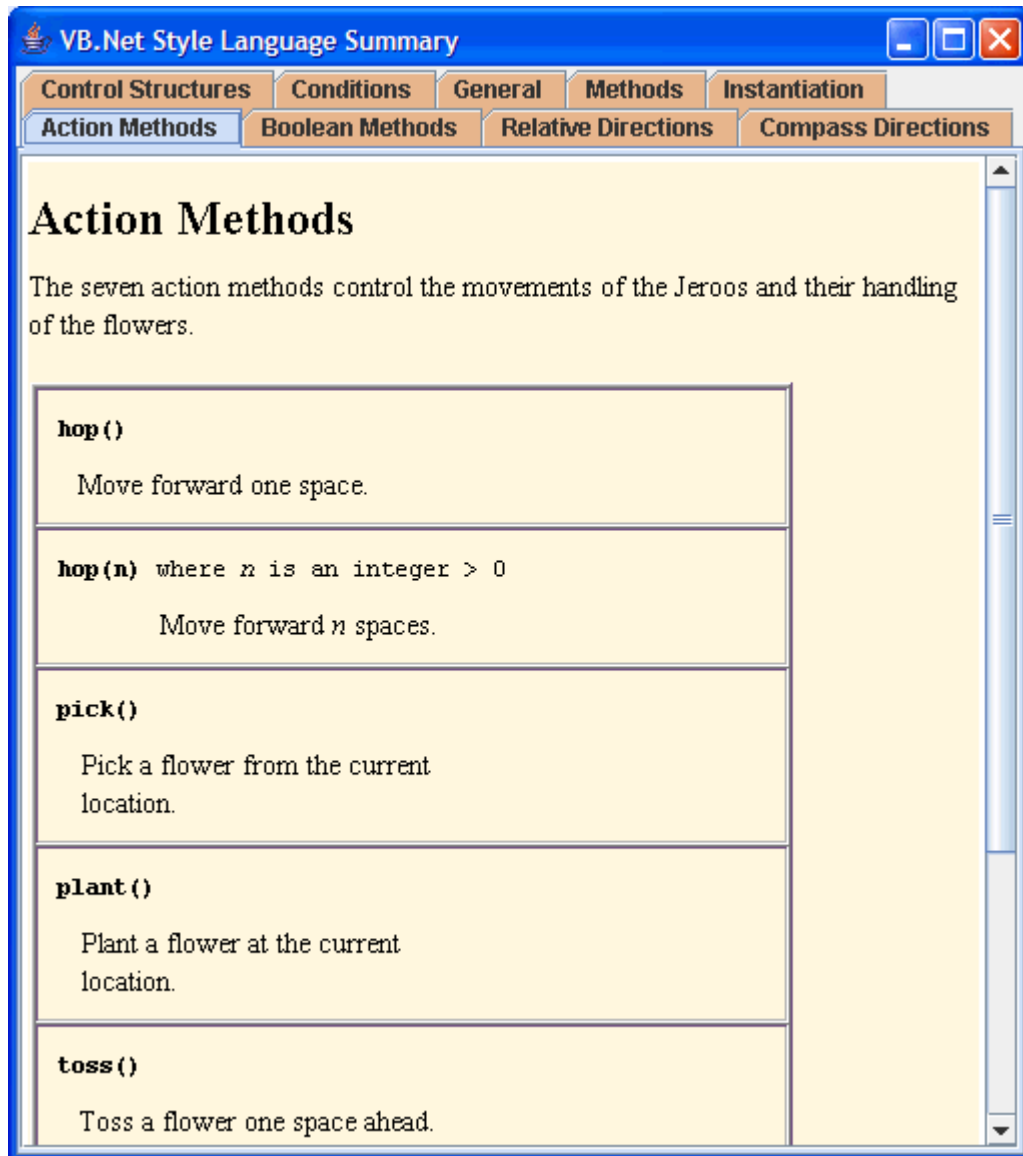
Figure C.15 – The VB.NET-Style Language Summary Window
