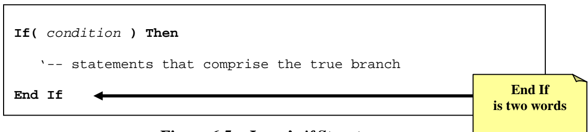
Figure 6.5 – Jeroo's if Structure
